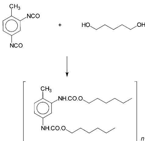
8.10 Polyurethane.
