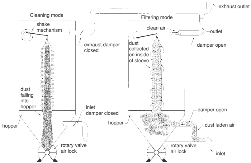
13.3 Shake collector.
