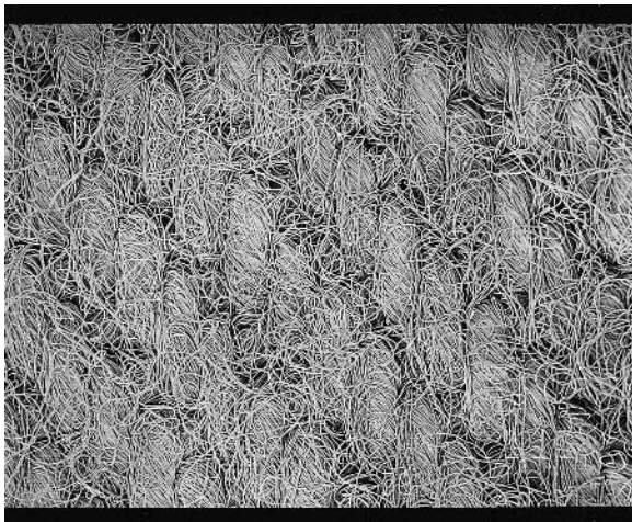
13.23 Scanning electron micrograph showing woollen ring-spun fabric.
