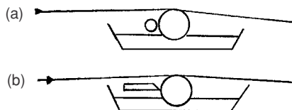
8.12 Other lick roll methods. (a) A metering roll and (b) a knife doctor.
