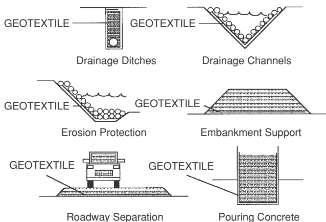
14.4 Some different drainage and filtration applications for geotextiles in civil engineering.
