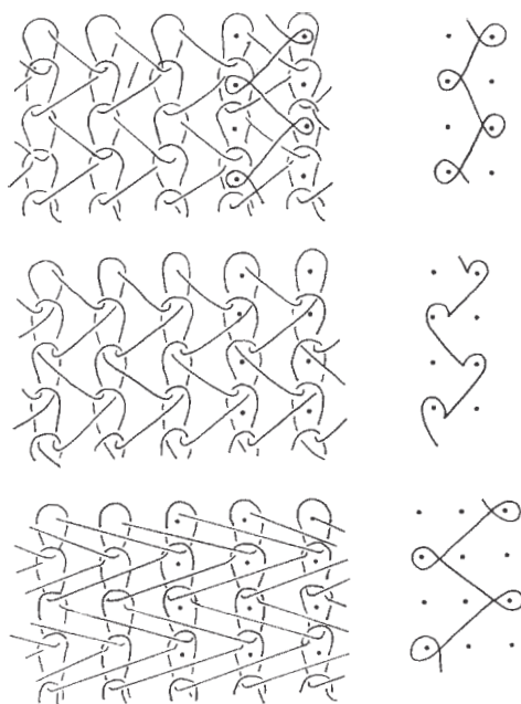
5.24 Single-guide bar structures.
