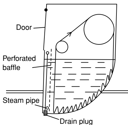
9.4 Winch dyeing machine (source: see ref 89, p. 38).
