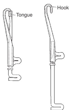
5.6 Compound needle (fly needle frame).
