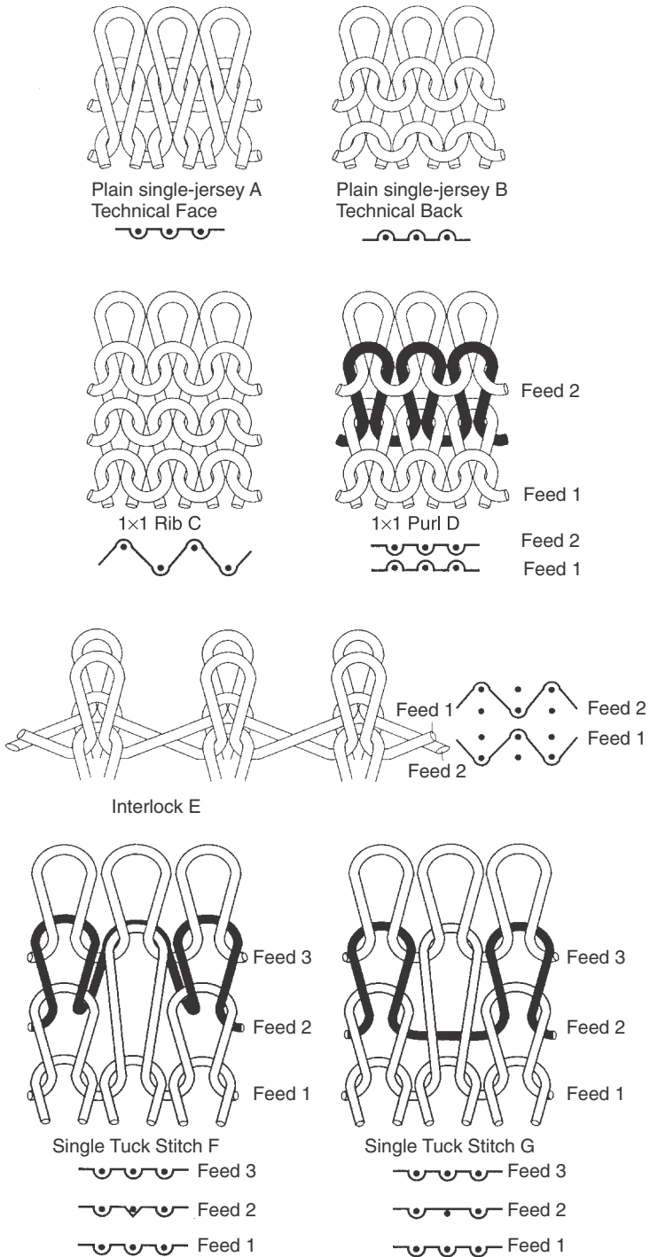
5.14 Weft-knitted structures (A–G).
