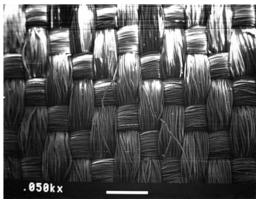
12.3 Scanning electron micrograph of microfilament fabric.
