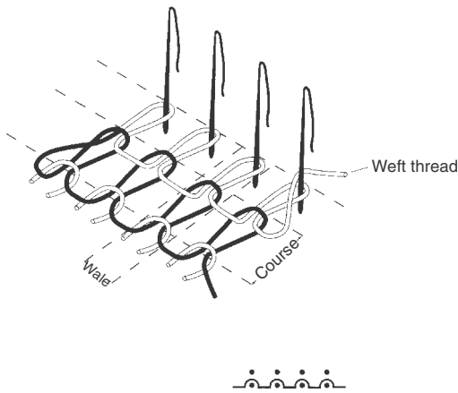
5.2 Weft knitting.
