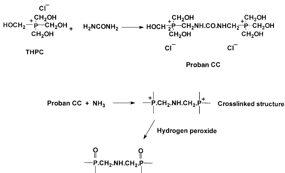
7.15 Chemistry of the Proban process.
