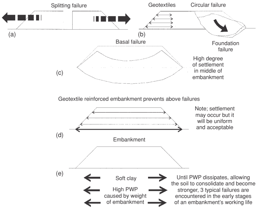
14.11 Short-term applications for geotextiles in embankments.
