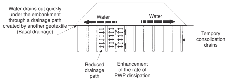
14.13 Temporary consolidation drains.
