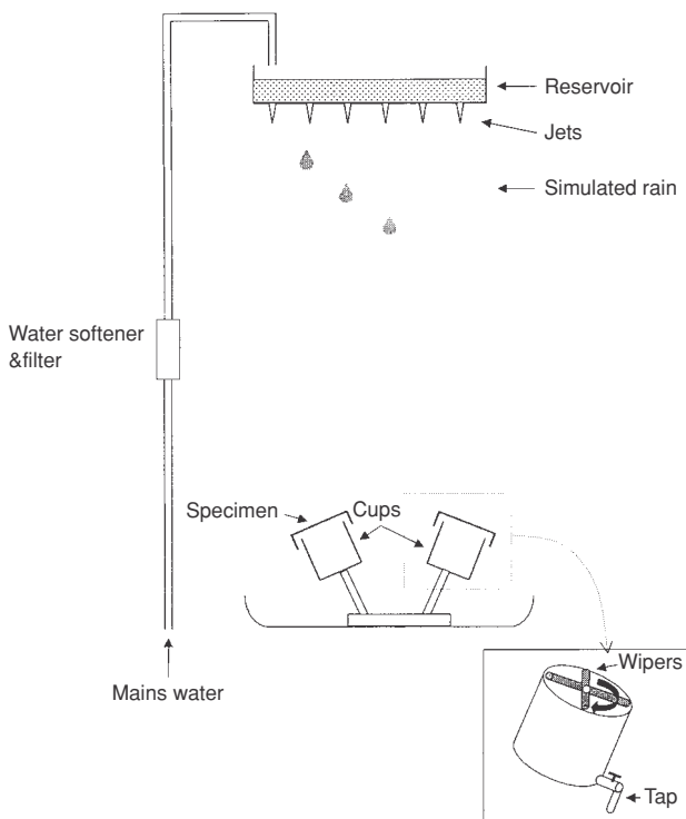
12.13 Diagram of Bundesmann apparatus.
