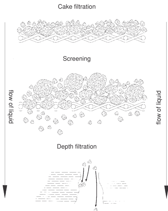
13.12 Solid/liquid filtration mechanisms.
