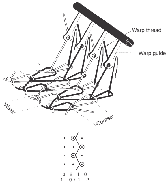
5.1 Warp knitting.
