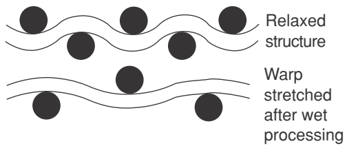
7.9 Fabric relaxation.
