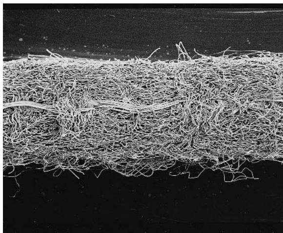
13.7 Scanning electron micrograph showing cross-section of needlefelt.
