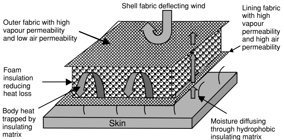
17.1 Construction of VÆTREX insulation system. 30
