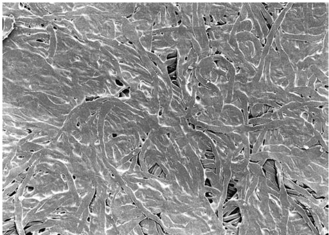
13.31 Scanning electron micrograph showing needlefelt with fused fibre surface.
