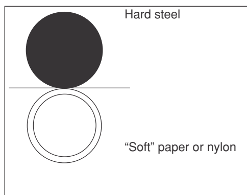
7.3 Two-bowl calender.
