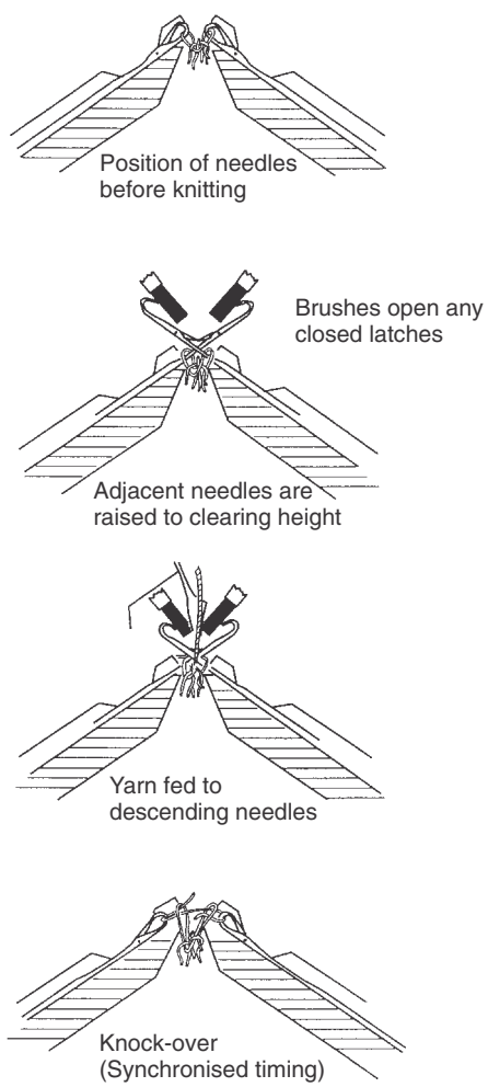
5.12 Loop formation on a V-bed flat knitting machine.
