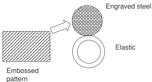
7.5 Principle of Schreiner calender.
