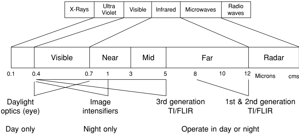
16.5 Electromagnetic spectrum. TI/FLIR = Thermal imaging/forward looking infrared.
