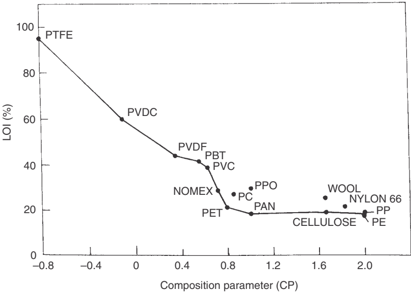
10.4 Correlation between oxygen index and elemental composition. PTFE = poly(tetrafluoroethylene), PVDC = polyvinylidene chloride, PBT = poly(butylene terephthalate), PVDF = polyvinylidene fluoride, PVC = poly(vinyl chloride), PET = poly(ethylene terephthalate), PC = polycarbonate, PPO = poly(phenylene oxide), PAN = poly(acrylonitrile), PP = polypropylene, PE = polyethylene.
