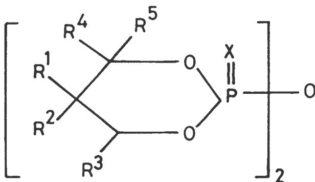
Structure II
