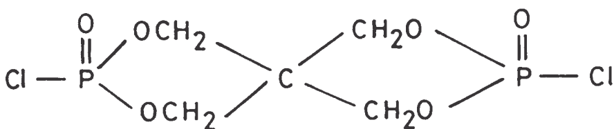
Structure III
