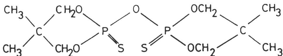
Structure I
