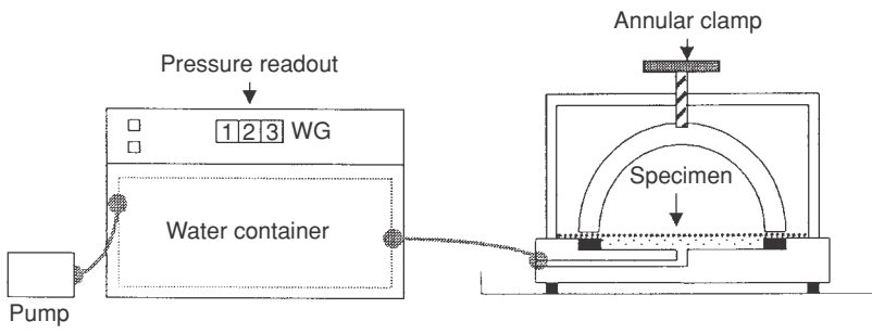
12.17 Diagram of hydrostatic head apparatus.
