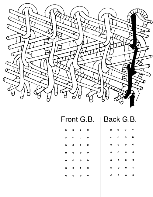
5.28 Three-needle queenscord.
