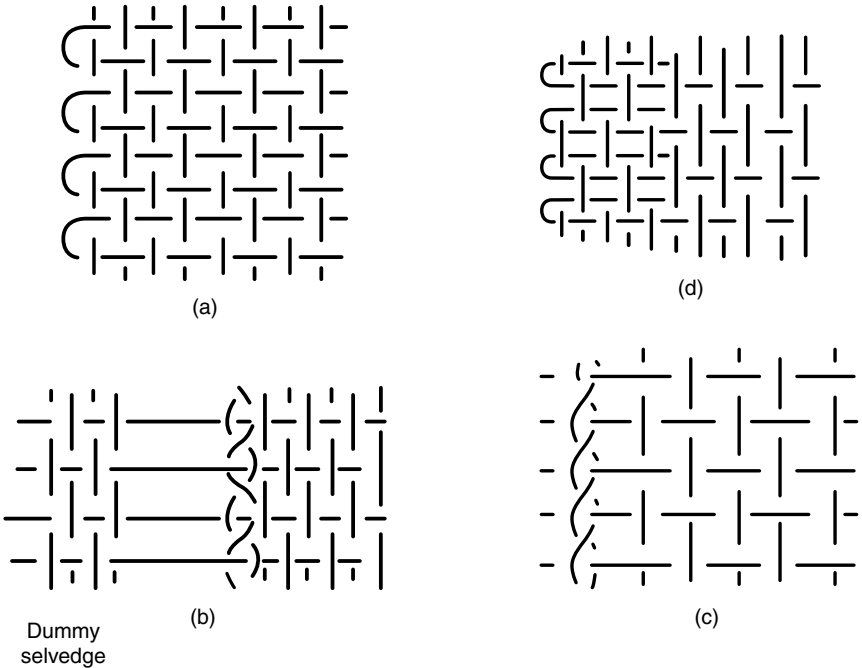
4.15 (a) Hairpin selvedge – shuttle loom, (b) leno selvedge with dummy selvedge, (c) helical selvedge, (d) tucked-in or tuck selvedge.
