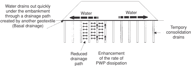
14.13 Temporary consolidation drains.
