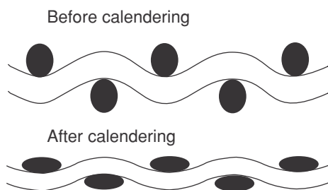
7.2 Flattening effect on fabric of calendering.
