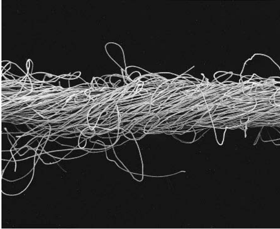
13.22 Scanning electron micrograph showing woollen ring-spun yarn.
