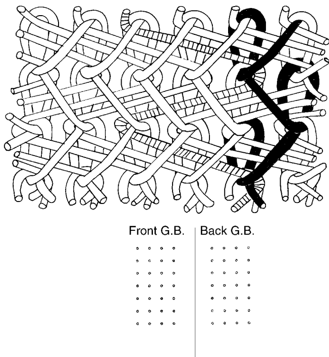
5.30 Laid-in structure.
