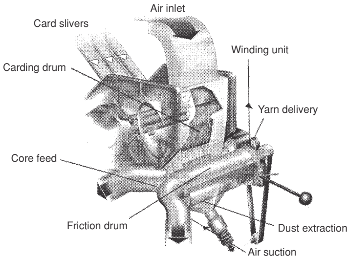
3.5 DREF 2 friction spinner.
