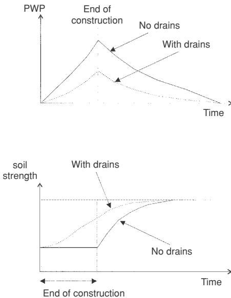
14.14 Comparison of time and strength of soil with and without consolidation drains.
