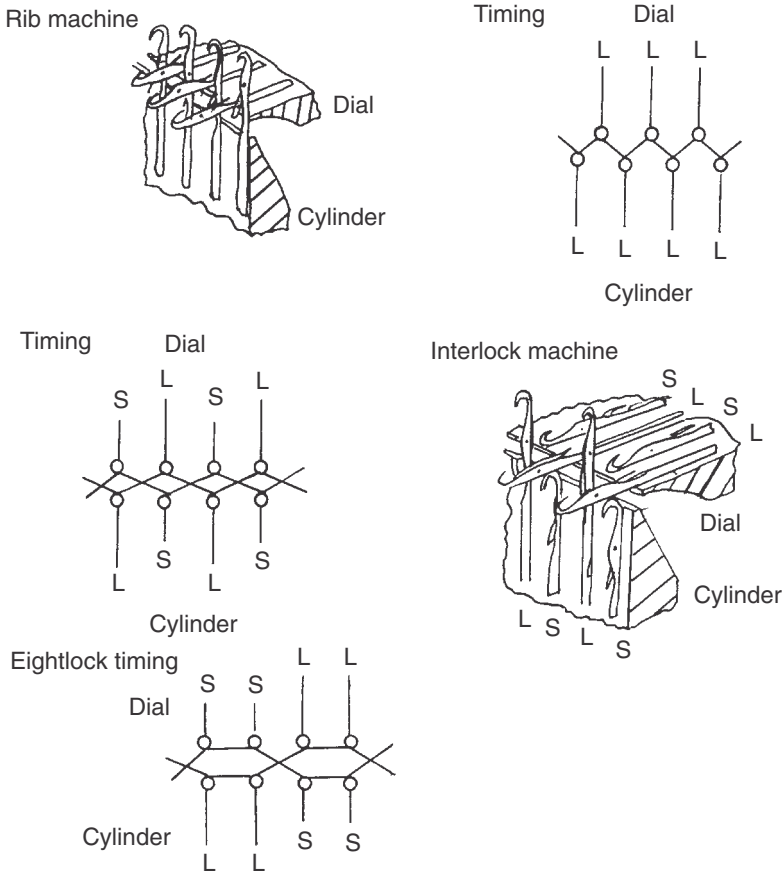
5.11 Double-jersey machine needle layouts.
