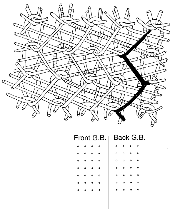
5.27 Three-needle sharkskin.
