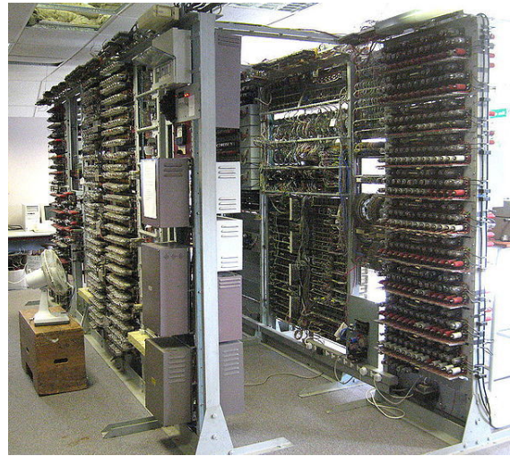
Colossus rebuild seen from the rear.
